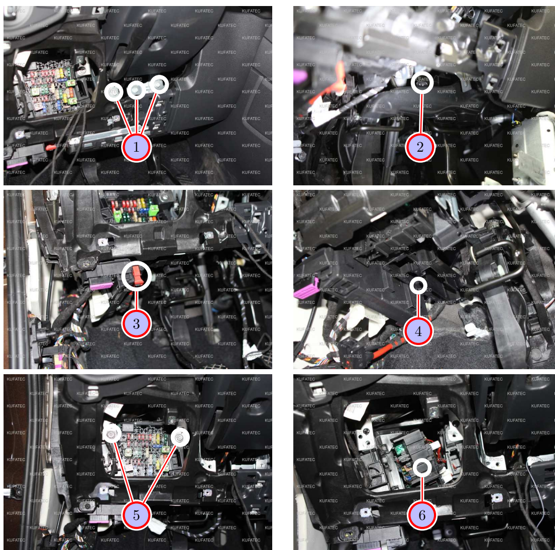
Figure 10: Removing fuse box
