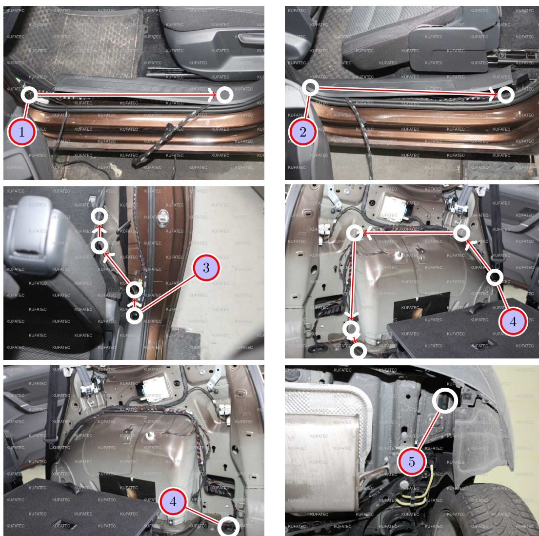
Figure 12: Cable routing
