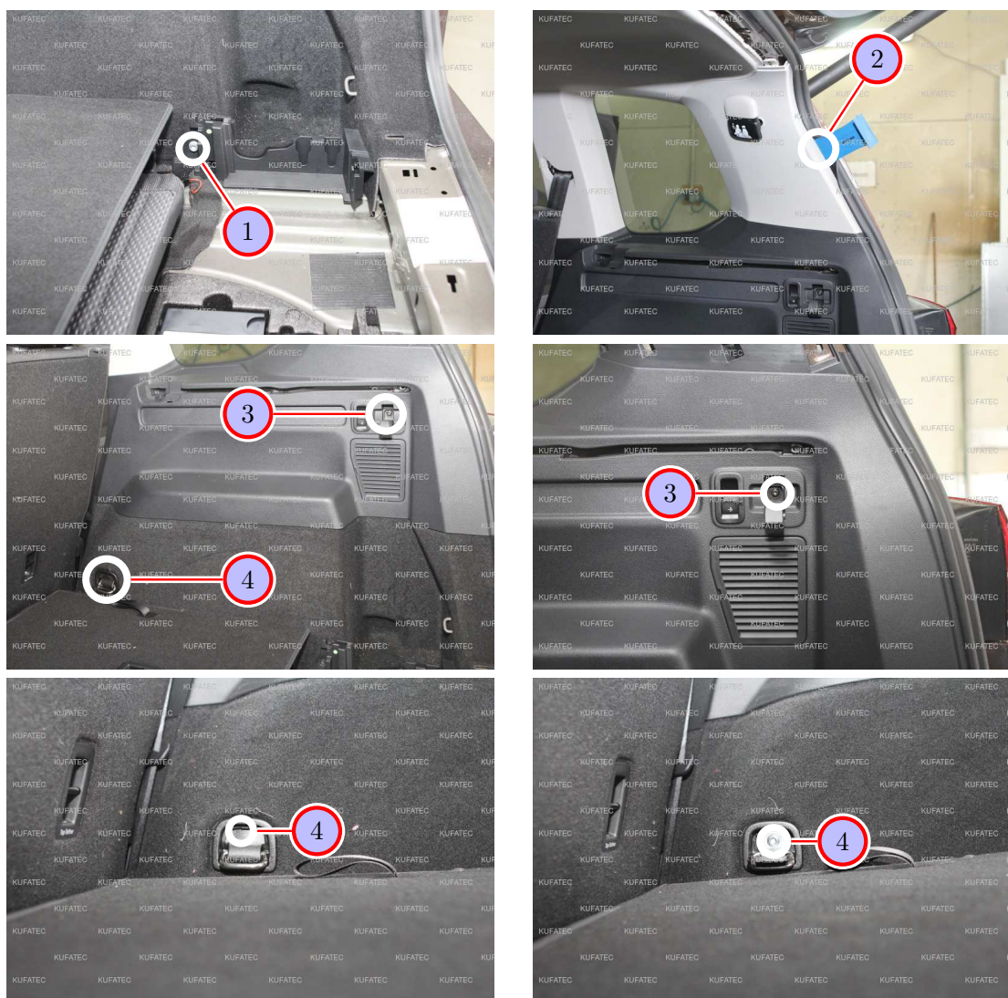
Figure 6: Removing trim panel car boot
