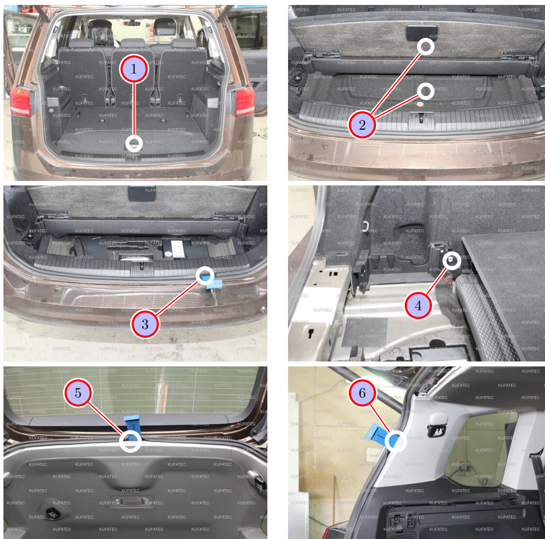
Figure 4: Removing trim panel car boot
