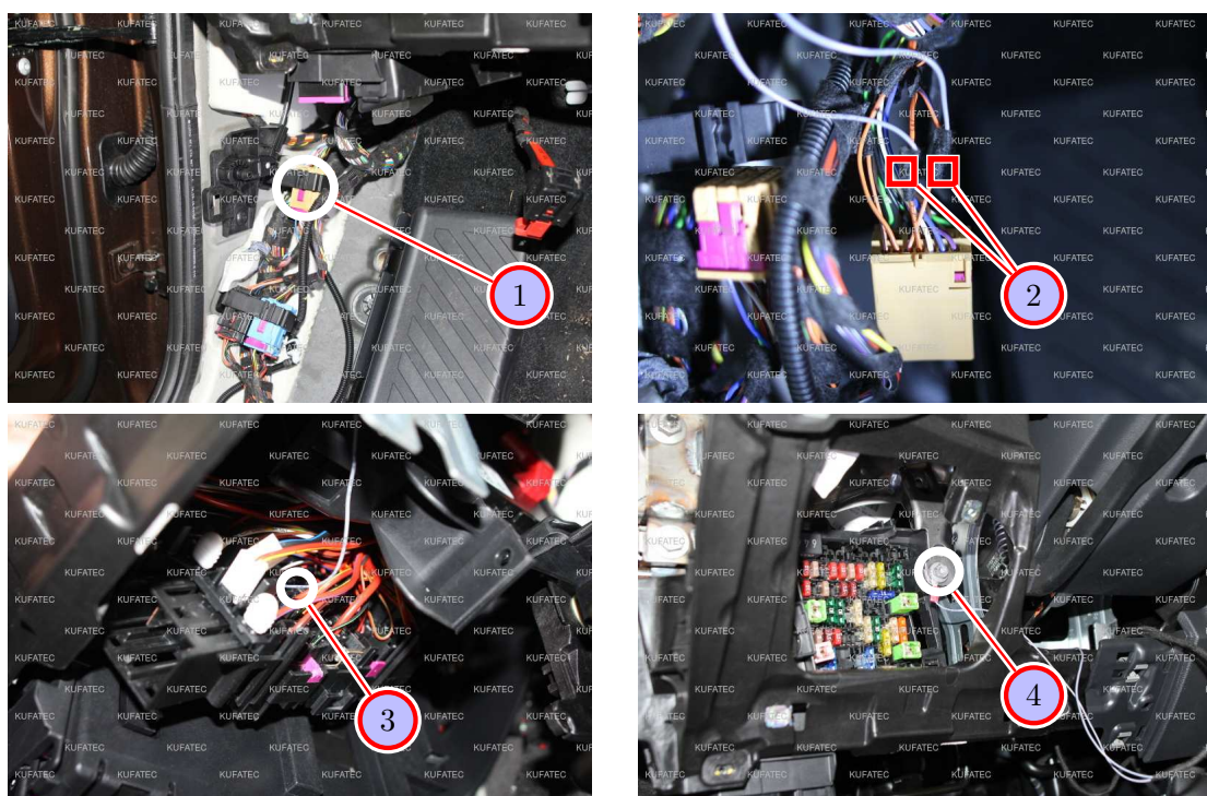
Figure 11: Connection CAN High/Low, ground and ignition plus
