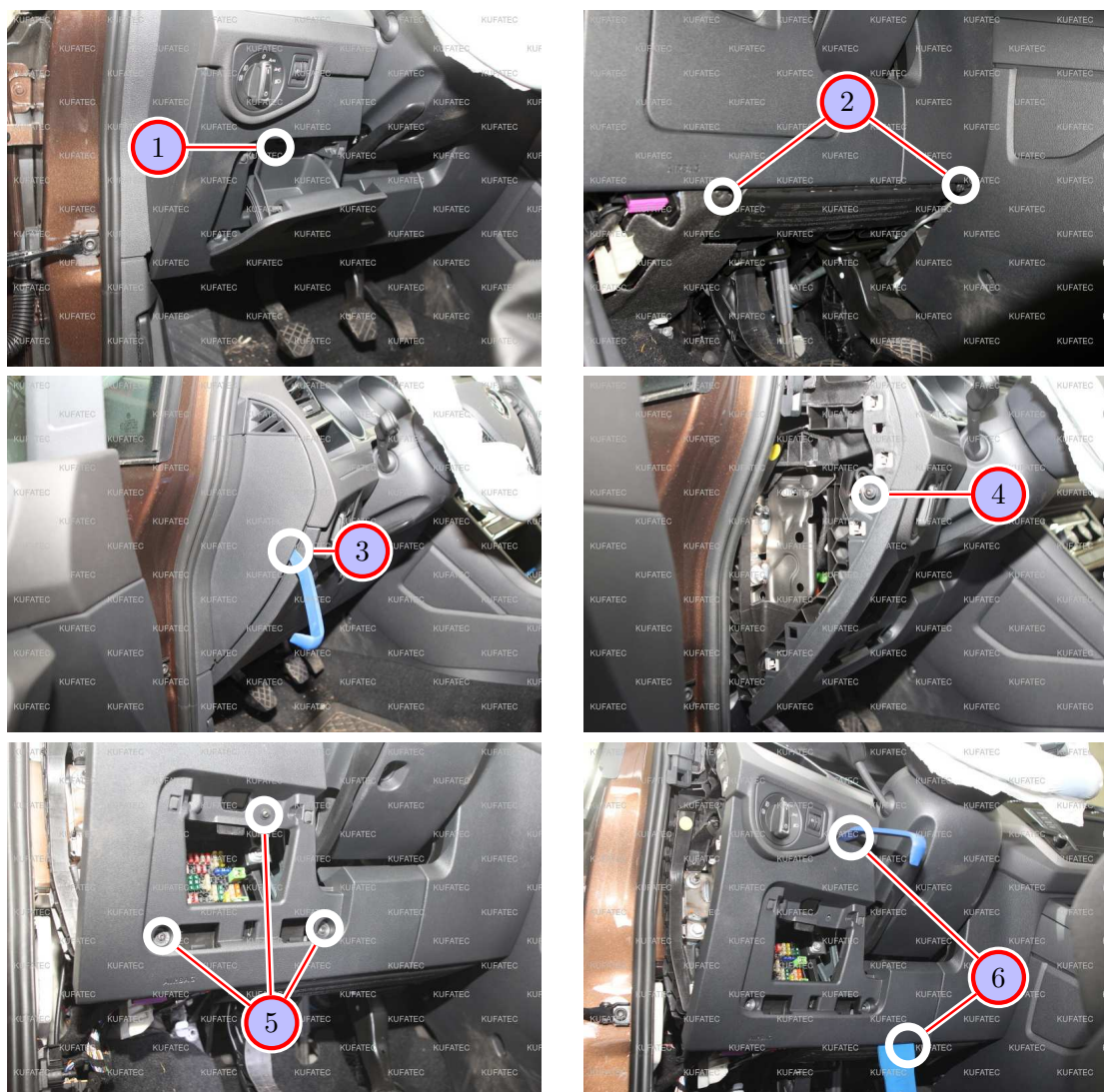
Figure 8: Removing trim panel driver's side
