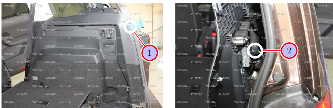
Figure 7: Removing trim panel car boot
