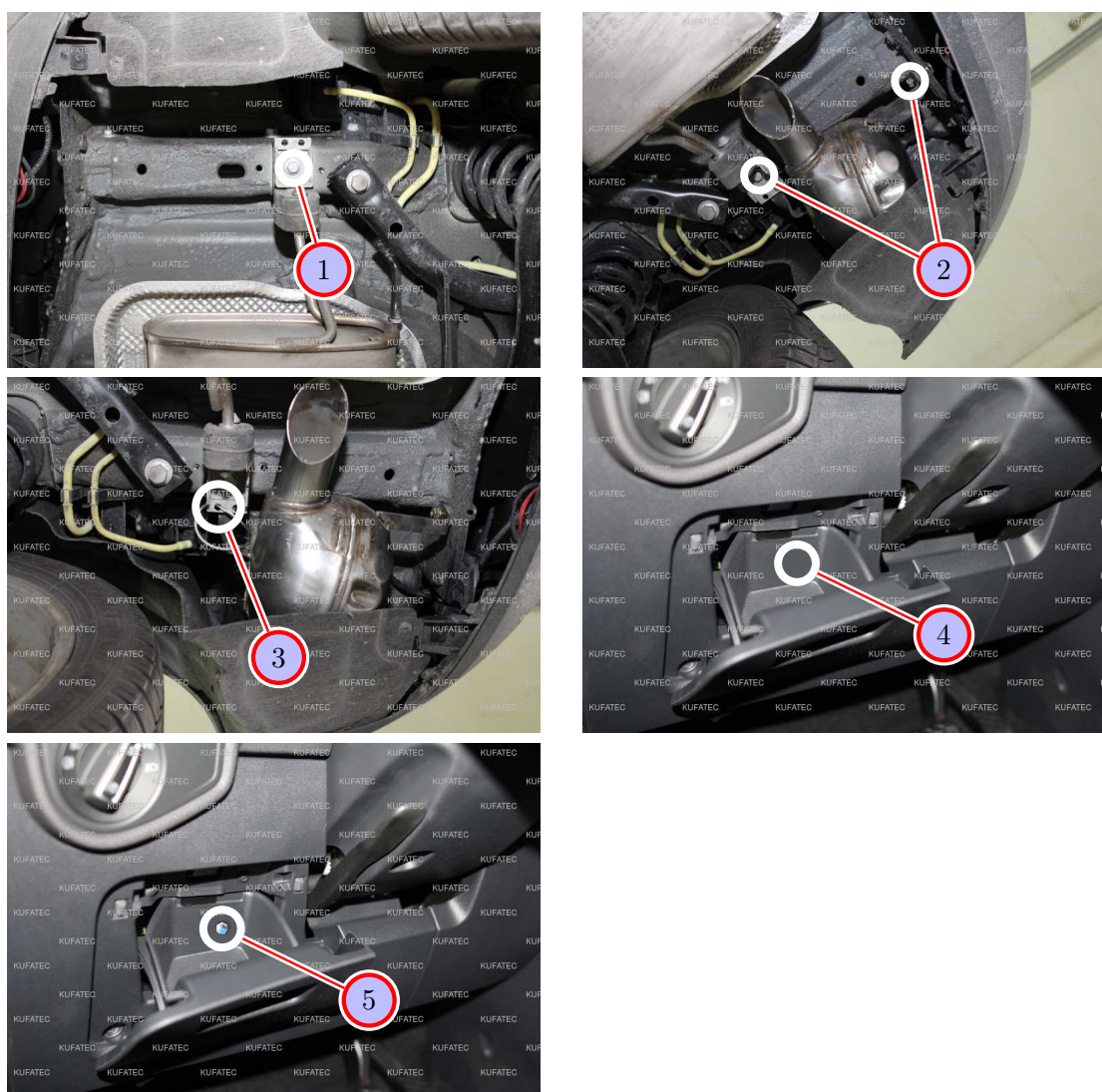
Figure 13: Sound generator and pushbutton installation
